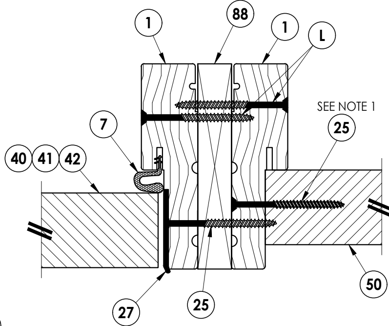
2 5 HORIZONTAL CROSS SECTION Shown w/ 2X Buck Outswing shown (Inswing similar)
