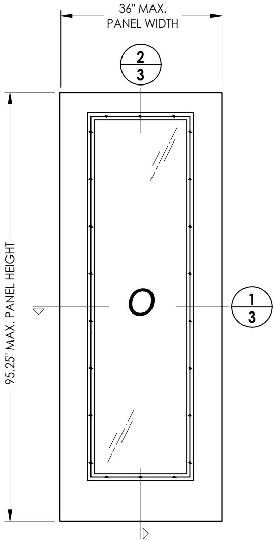
50 SIDELITE PANEL
